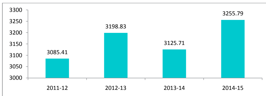
Diagram 1: GCF in Agriculture and Allied Sector (Rs. In crore)
